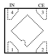
DFNWB1*1-4L (TOP VIEW)
