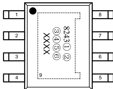
ESOP-8L (TOP VIEW)
