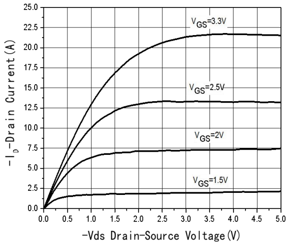
Fig1 Output Characteristics
