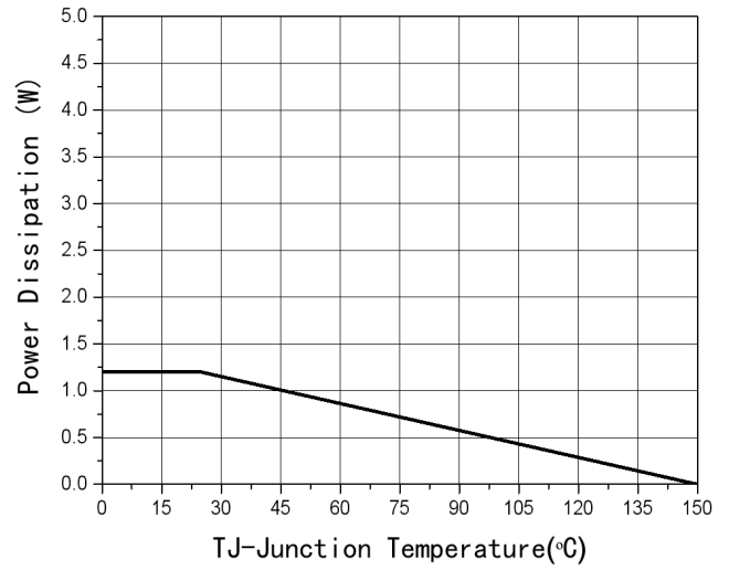
Fig8 Power De-rating
