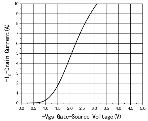
Fig2 Transfer Characteristics
