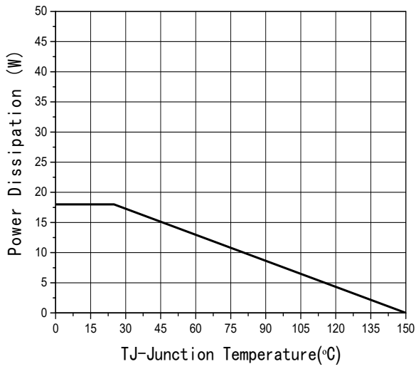
Fig7 Power De-rating
