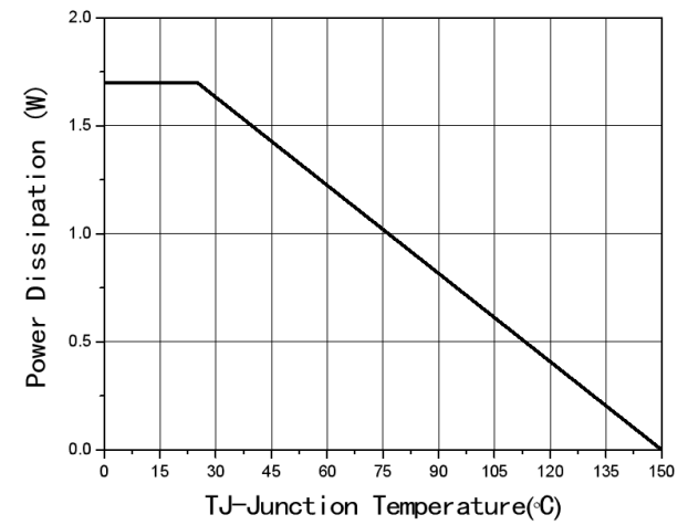
Fig8 Power De-rating
